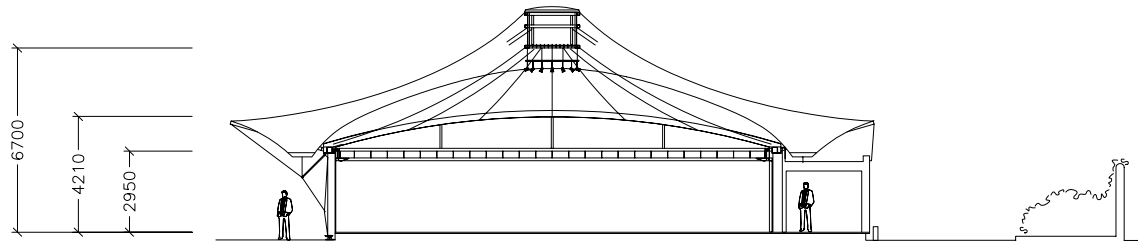
SECTION B-B
